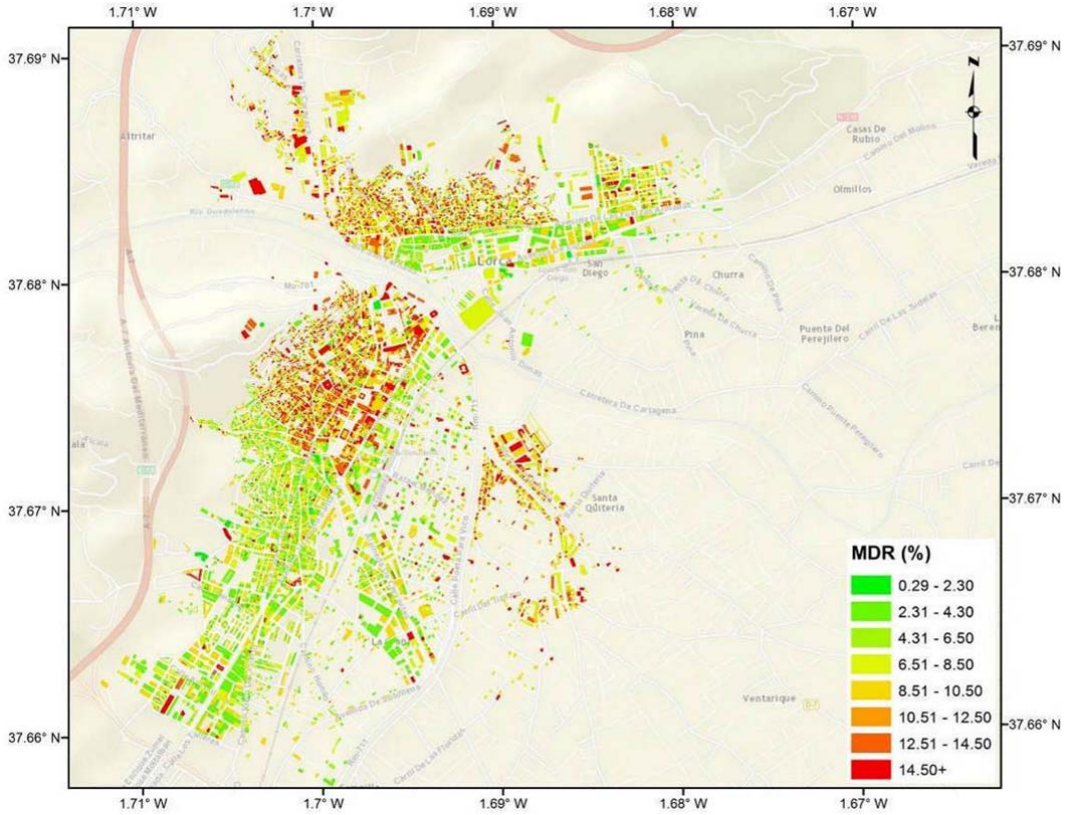
Figure 2. MDR distribution for the modelled scenario in Lorca
