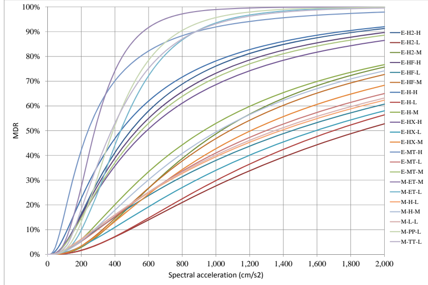
Figure 1. Vulnerability functions used for the buildings in Lorca (L=Low-rise; M=Medium-rise; H: High-rise)
